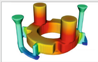
CASTING SIMULATION
