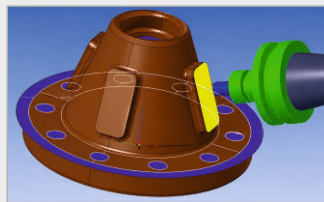
MACHINING SIMULATION
